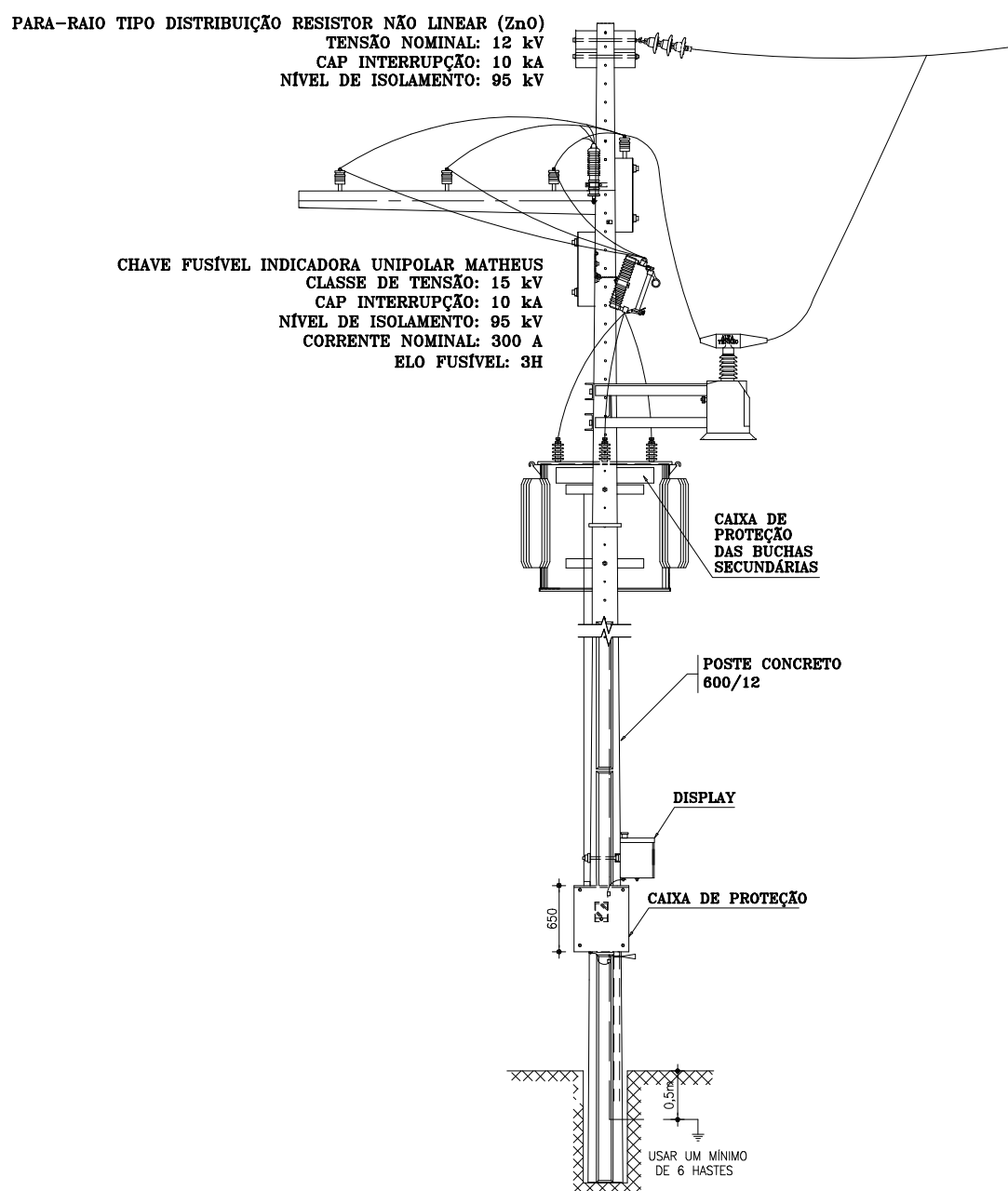
3 VISTA FRONTAL ESCALA 5/8"
