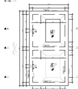
FÔRMA – PLANO 4-4
