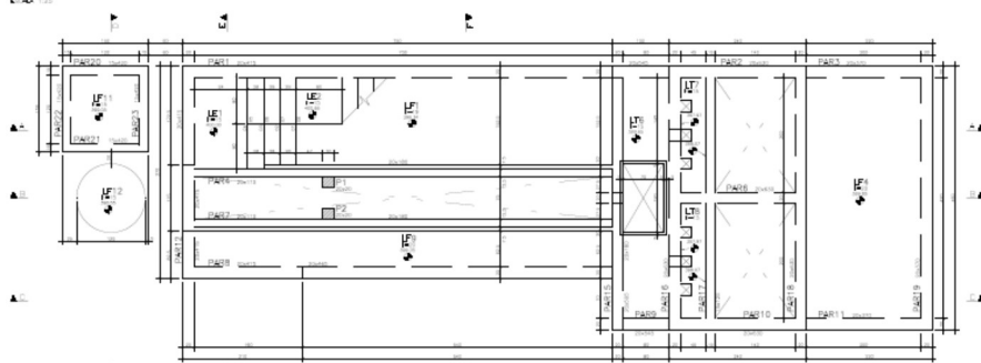
FÔRMA – PLANO 3-3
