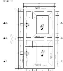
FÔRMA – PLANO 4-4 E=4/1,00
